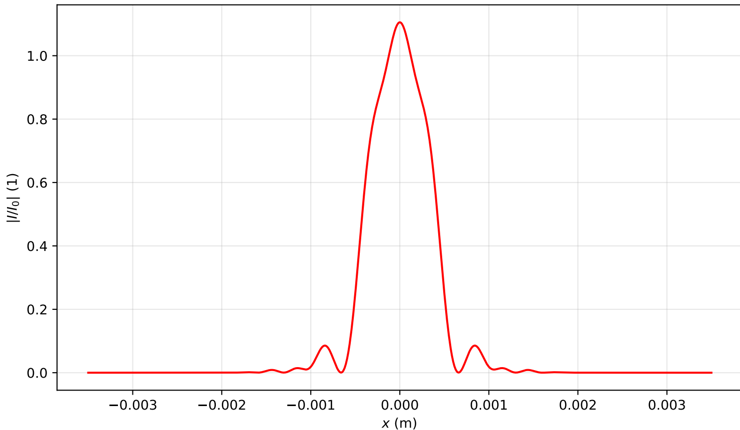
Intensity profile I(x, y = 0, z = 1.433)/I_0 , P_{in}=2.5P_{cr} , artificial time
